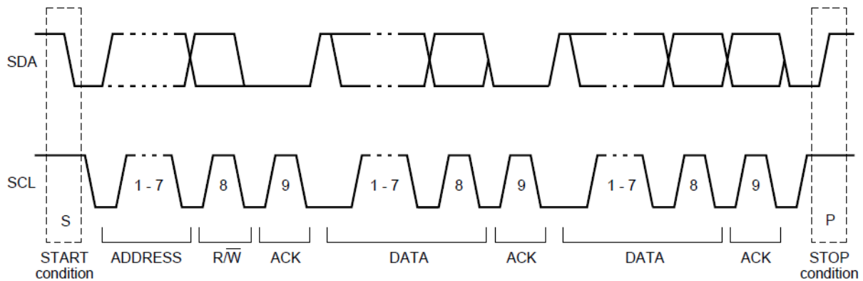
Figure 10-2 I2C Timing
