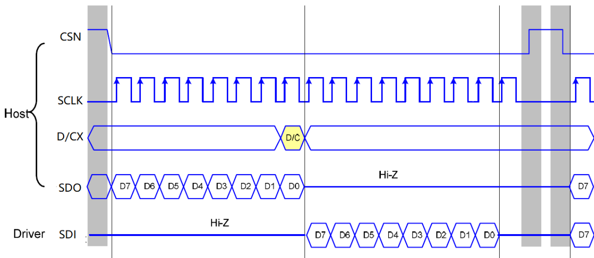
Figure 10-12 4-Line Read Sequence
