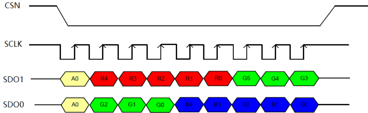
Figure 10-15 RGB666 Pixel Transition
