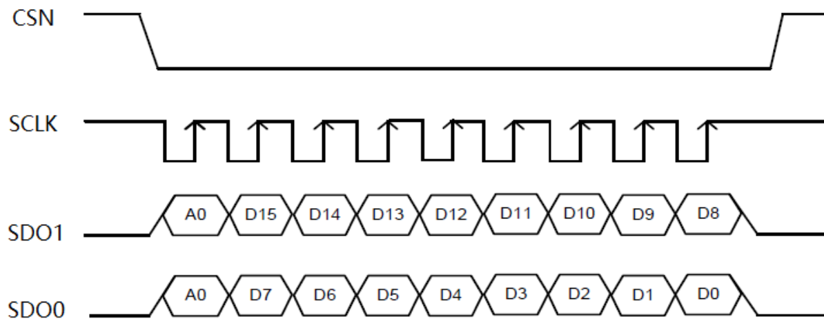
Figure 10-13 2-Line Write Sequence
