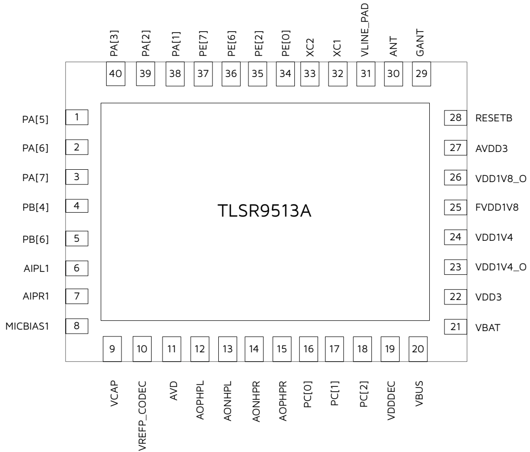
Figure 1-4 Pin Assignment of TLSR9513A
