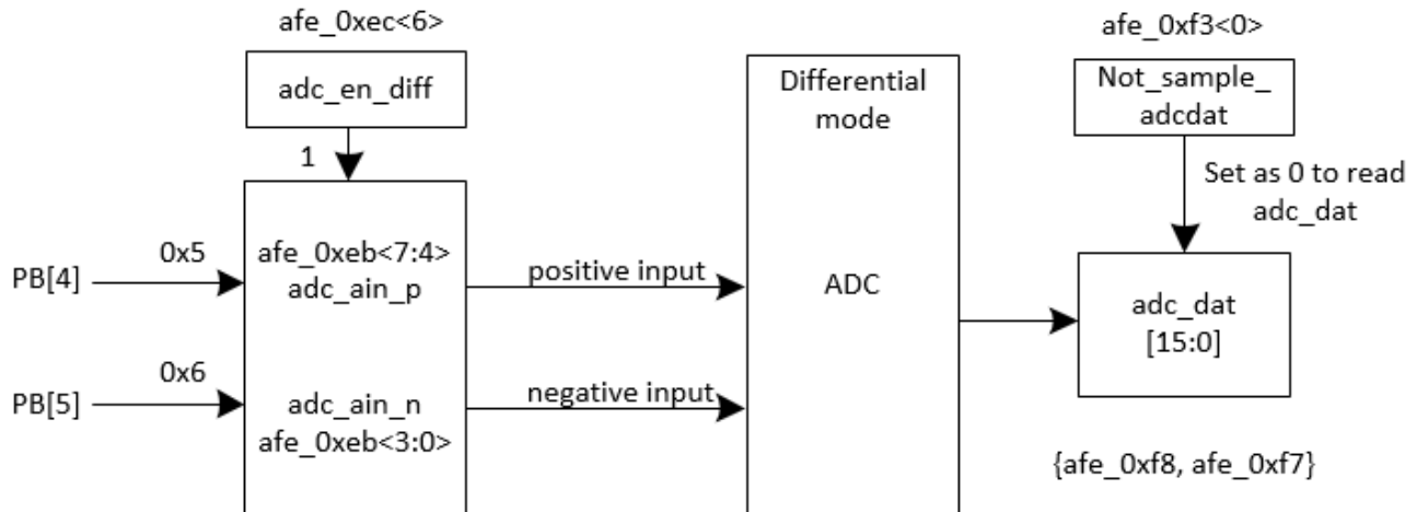
Figure 12-1 Diagram of ADC
