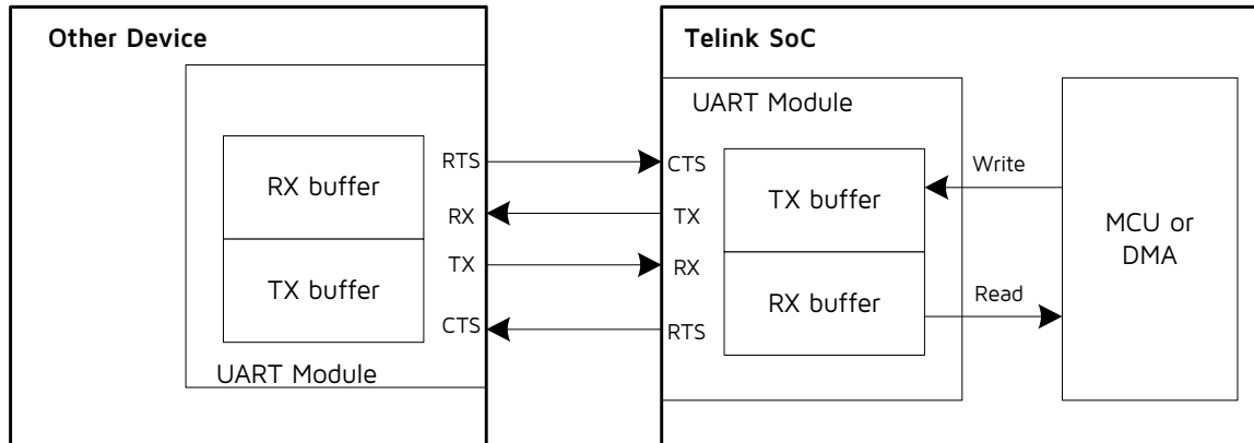
Figure 10-17 UART Communication
