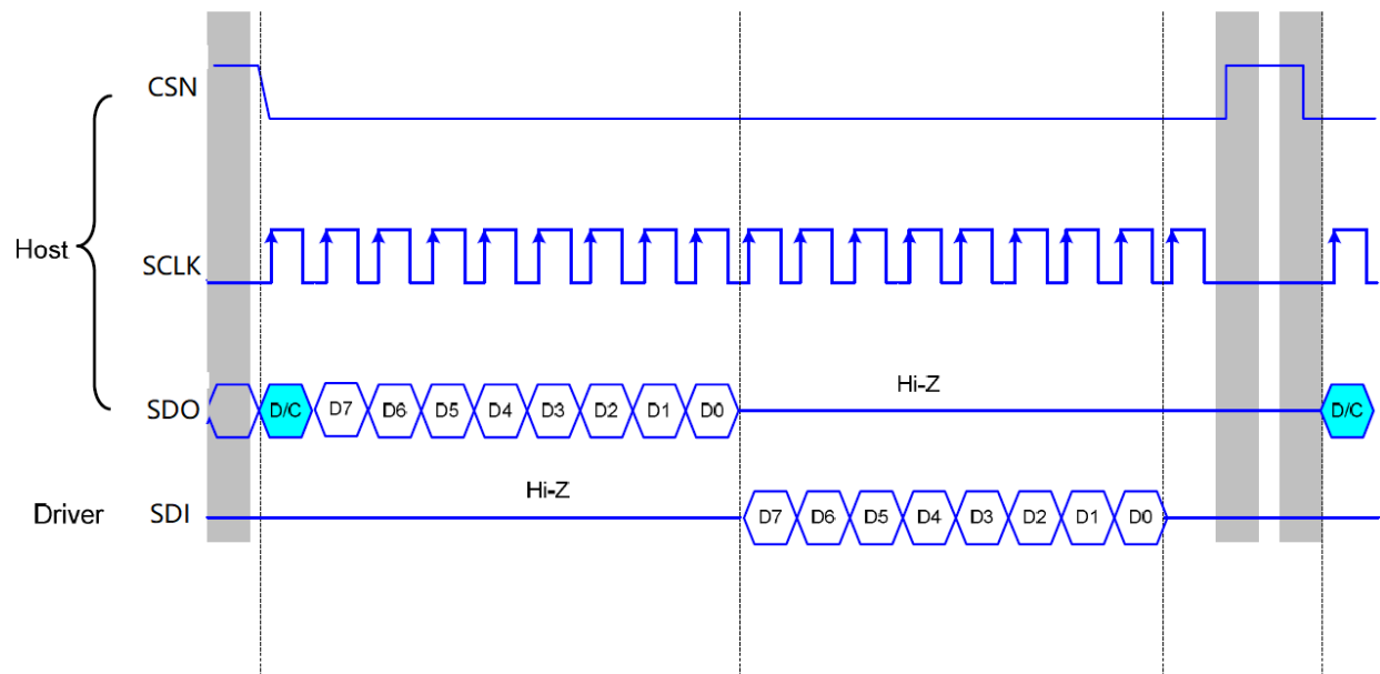
Figure 10-11 4-Line Write Sequence
