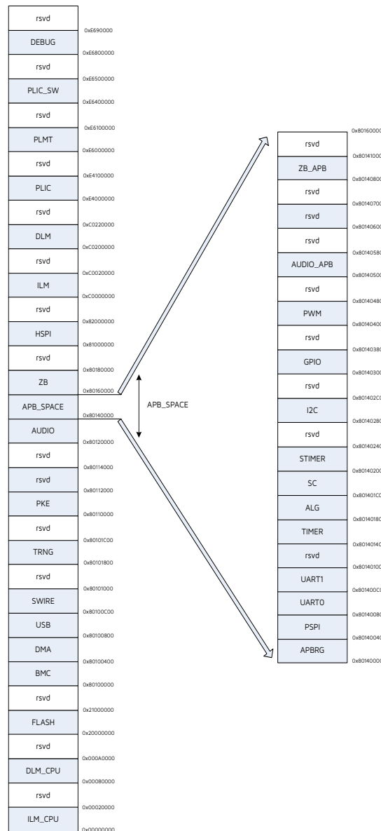
Figure 4-1 Memory Map
