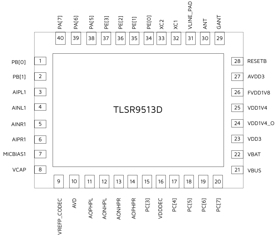
Figure 1-6 Pin Assignment of TLSR9513D
