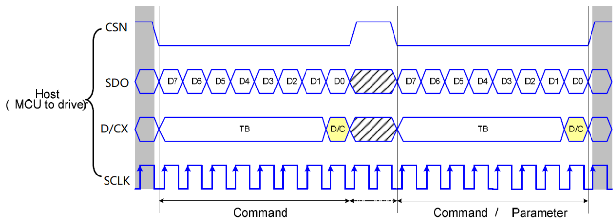
Figure 10-11 4-Line Write Sequence
