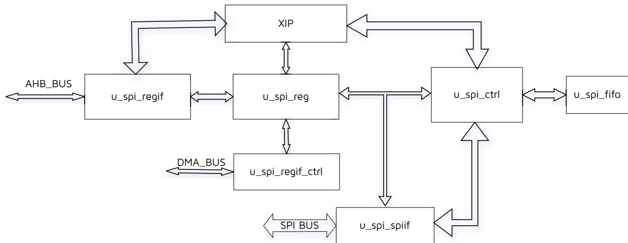
Figure 10-6 HSPI Diagram
