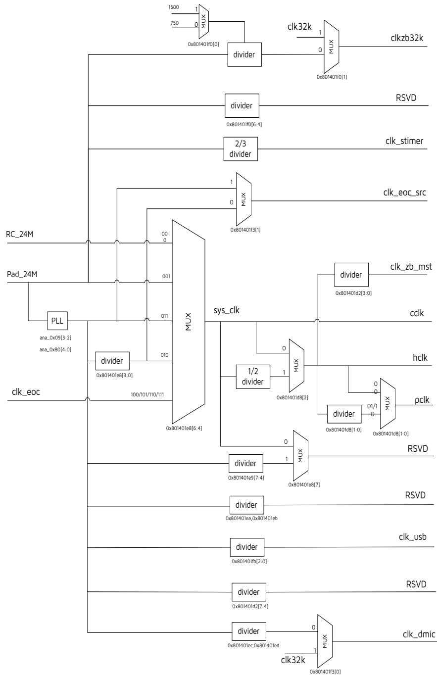
Figure 7-1 Clock Source
