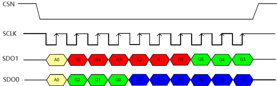
Figure 10-16 RGB888 Pixel Transition
