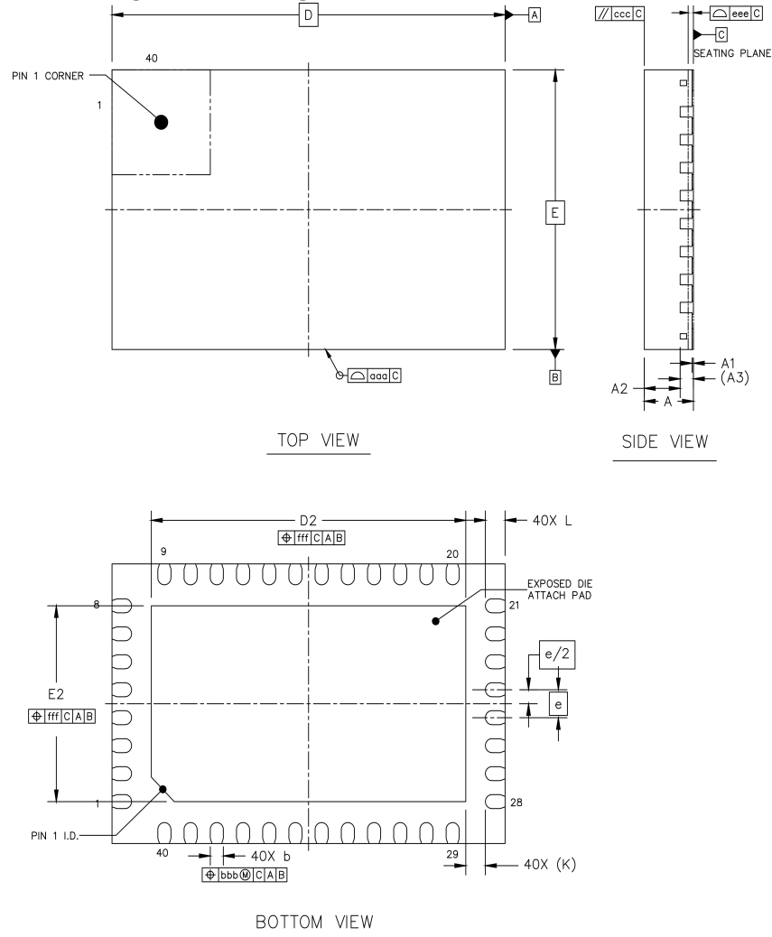
Figure 1-3 Package of TLSR9513B and TLSR9513D
