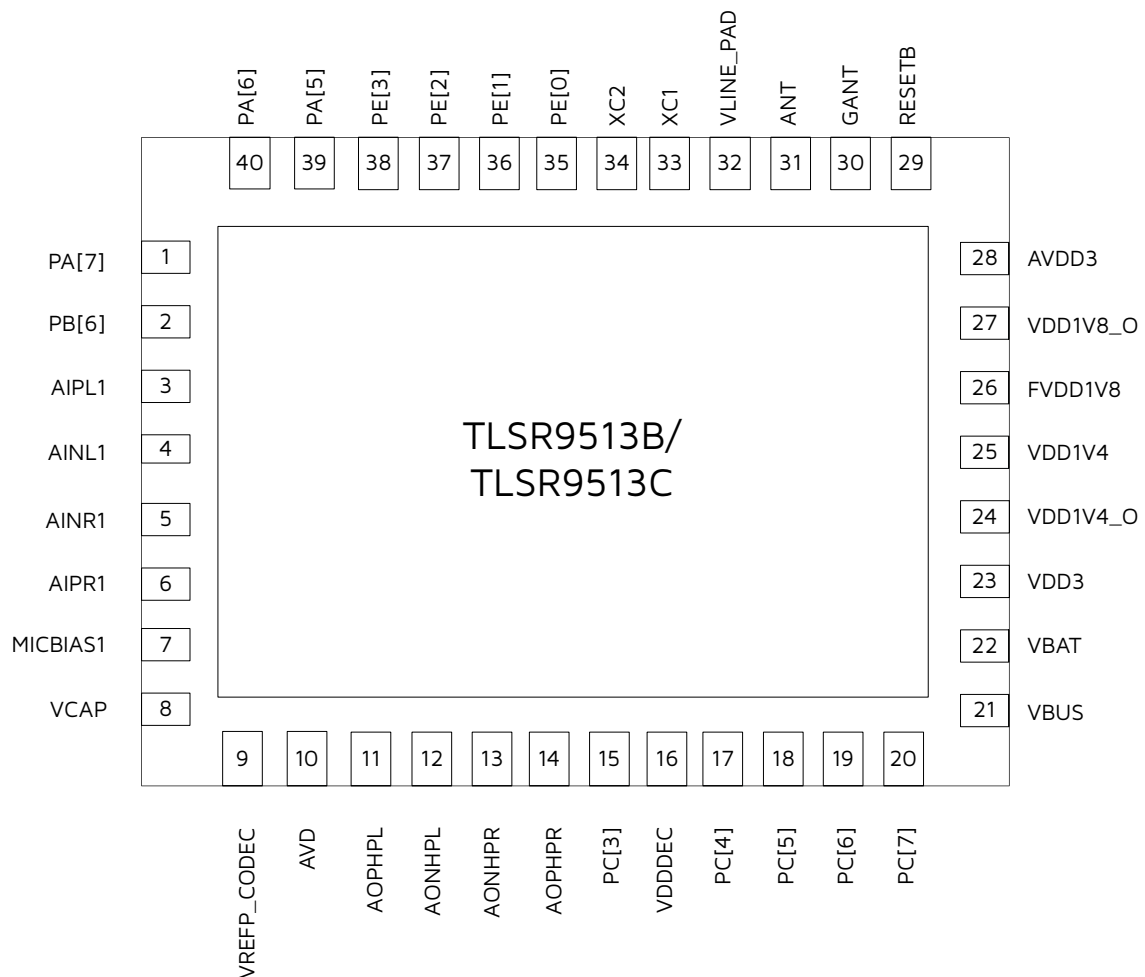
Figure 1-5 Pin Assignment of TLSR9513B/C
