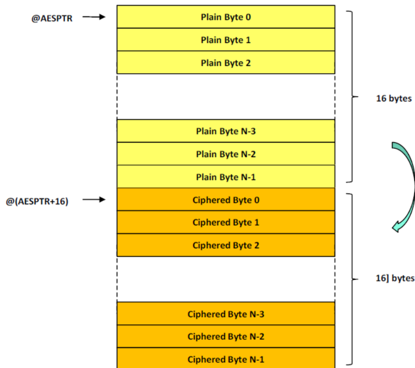
Figure 15-1 AES Address
