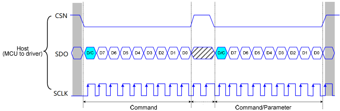
Figure 10-9 3-Line Write Sequence
