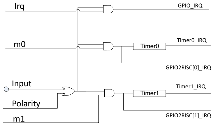
Figure 10-1 Logic Relationship between GPIO and Related Modules
